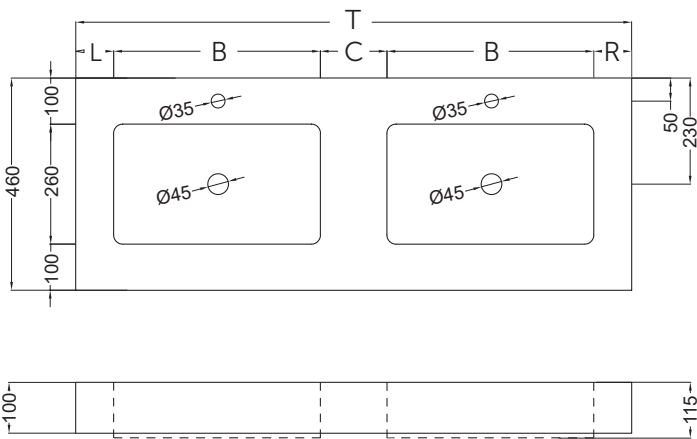
Washbasin Toren double basin 120 - 200
